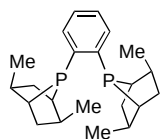
( R,S,R,S )-Me-PennPhos
